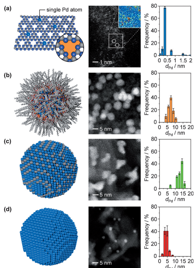
Figure 1. a–d) Structure of the materials (left), aberration-corrected scanning transmission electron microscopy images (middle), and particle size distribution (right) of [Pd]mpg-C 3 N 4 (a), Pd-HHDMA/TiS (b), Pd-Pb/CaCO 3 (c), and Pd/Al 2 O 3 (d). The structures depict the increasing size of the active ensemble, from a single Pd atom (a) to a bare Pd nanoparticle of approximately 800 atoms (d). The inset in (a) shows a characteristic six-fold cavity in the carbon nitride structure, which is crucial for confining palladium atoms in a stable manner. The two-dimensional Gaussian function modeling of a selected region of [Pd]mpg-C 3 N 4 is shown in the inset of the micrograph in (a) to enable visualization of the single Pd atoms (in red). C dark gray, H white, N purple, O red, P light orange, Pb light gray, Pd blue.
